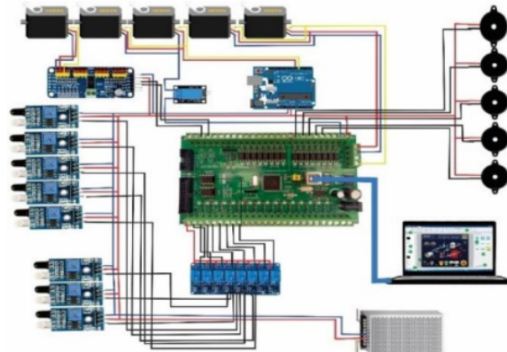
Gambar 4. Wiring Diagram
