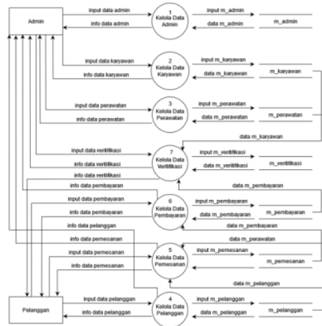
Gambar. 6. DFD level 1
