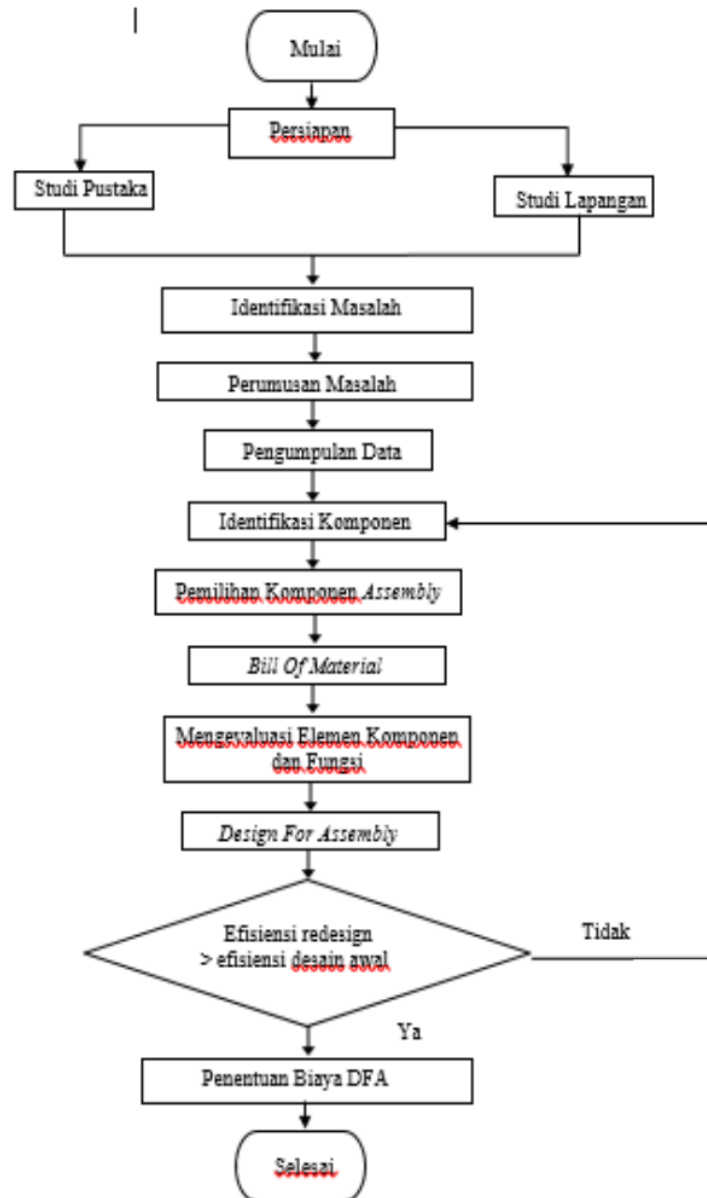
Gambar 1. Flowchart Penelitian
