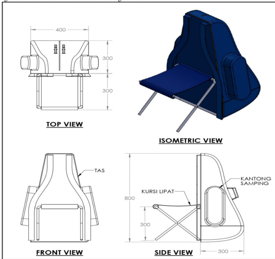
Gambar 4. Design Ukuran Detail Tas Pancing Multifungsi
