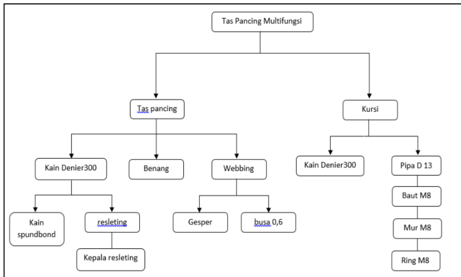
Gambar 3. Bill Of Material Tas Pancing Multifungsi
