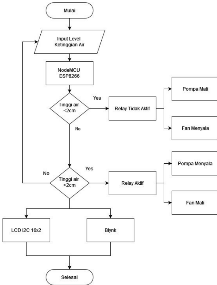
Figure 3. Flowchart sistem
