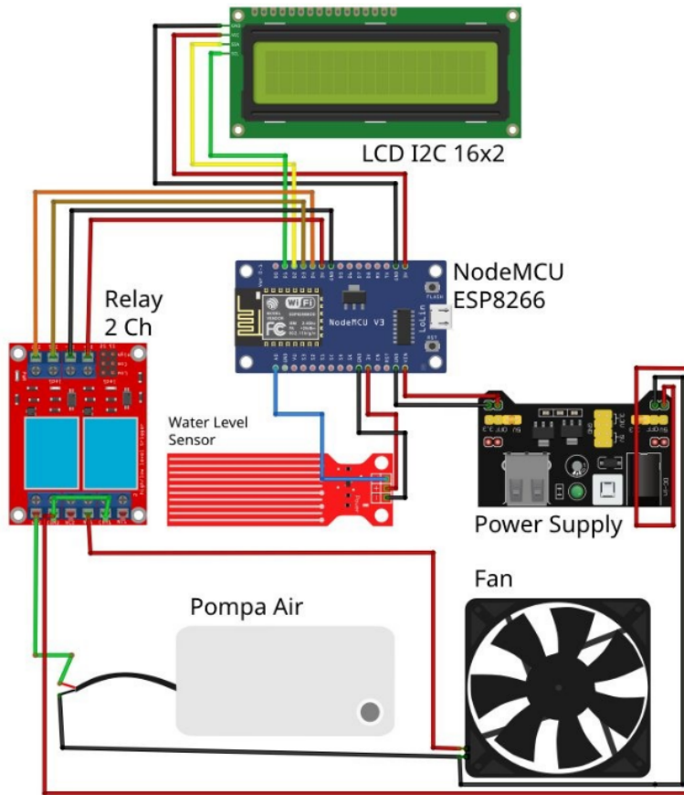
Figure 4. Wiring Diagram
