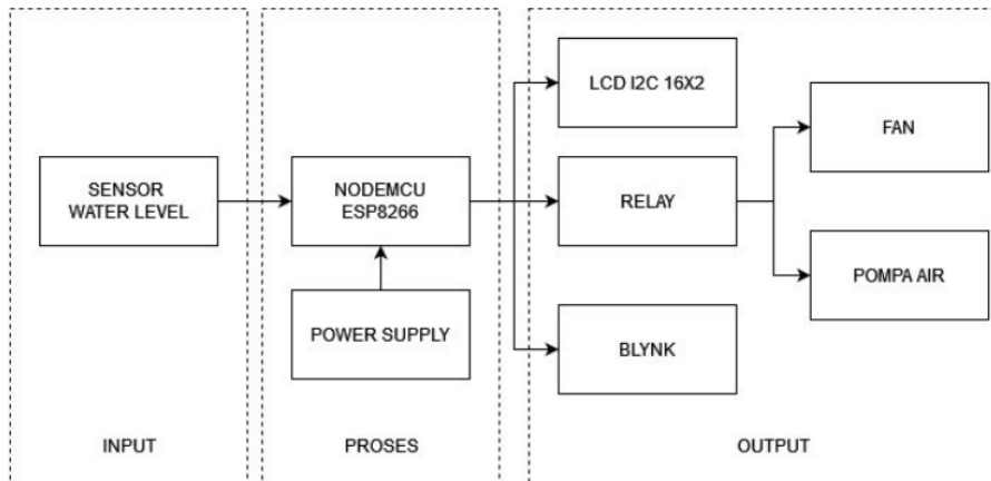
Figure 2. Diagram Blok
