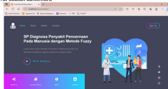
Gambar 15. Dashboard
