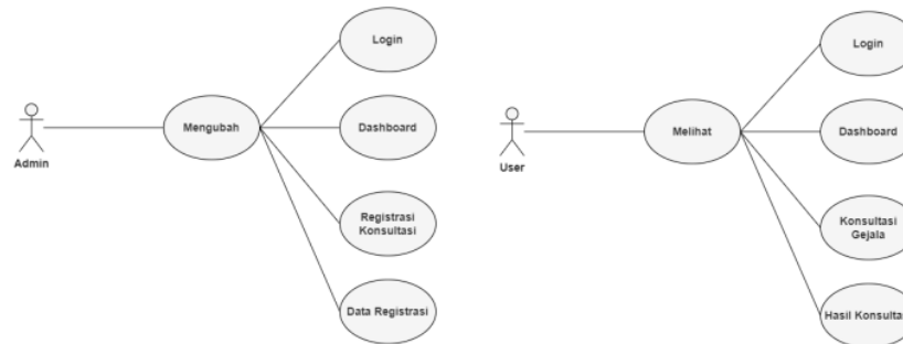
Gambar 5. Usecase Diagram
