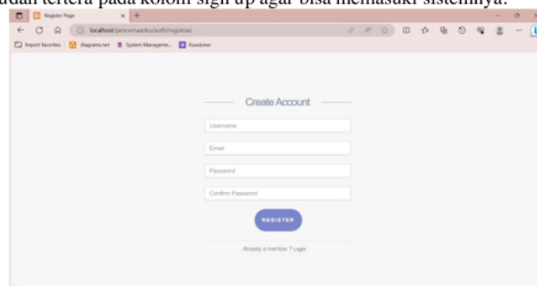
Gambar 7. Sign Up
