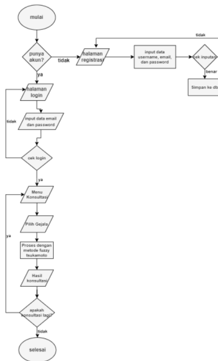
Gambar 2. Flowchart
