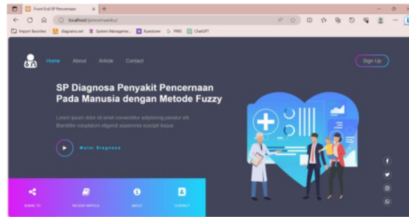
Gambar 6. Dashboard
