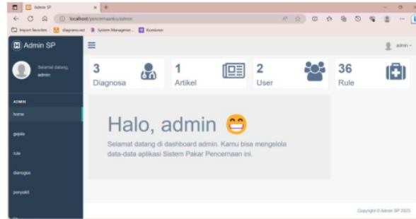
Gambar 9. Dashboard Admin
