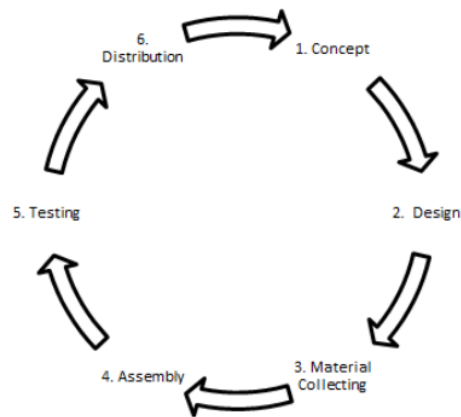
Gambar 1. MDLC
