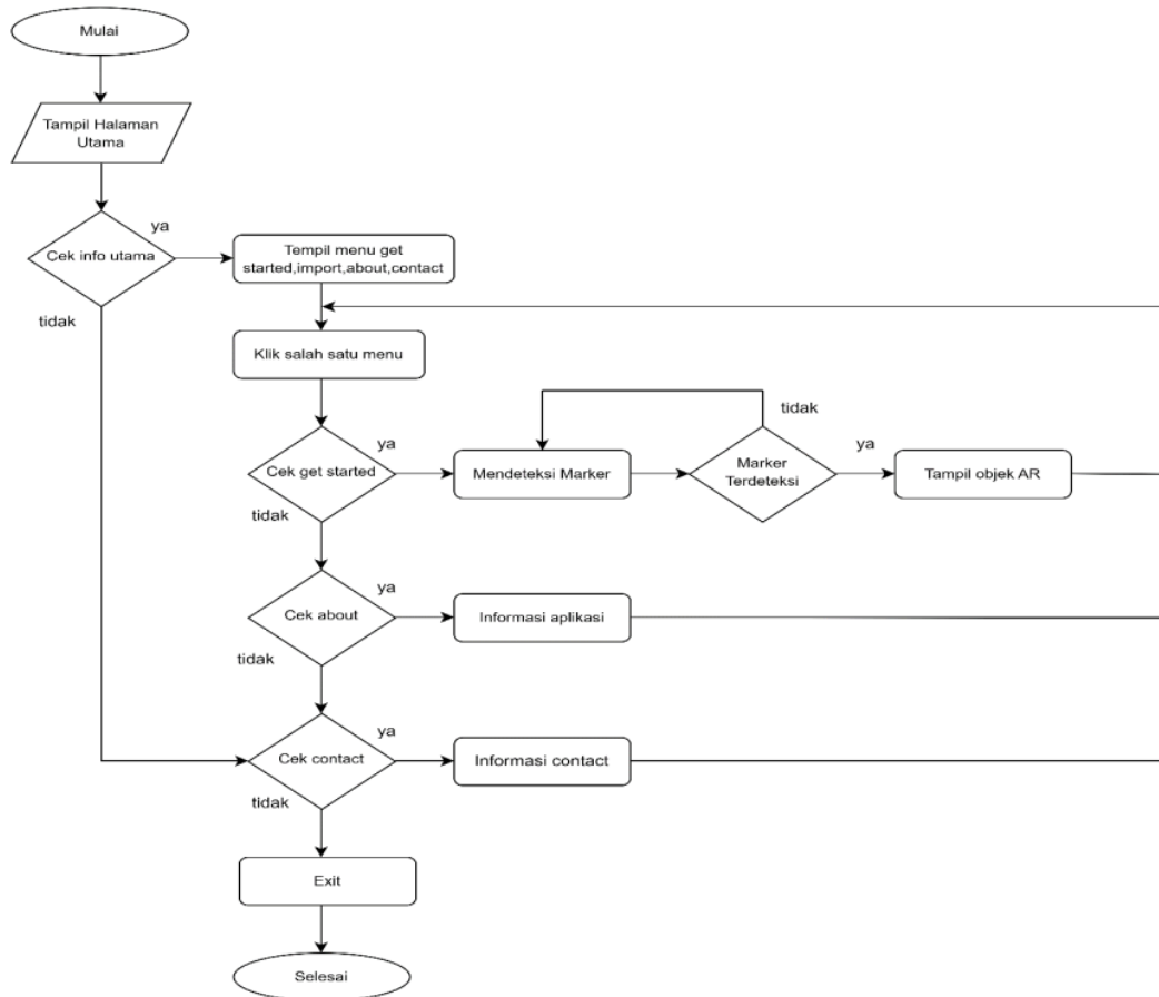
Gambar 2. Flowchart
