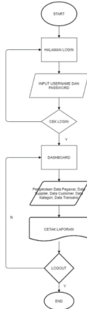
Gambar 2. Flowchart
