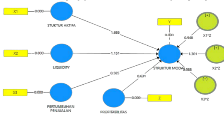
Gambar 1. Model Struktural Outer Model
