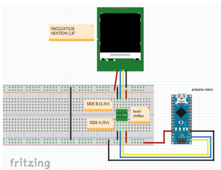
Gambar 7. Koneksi wiring Nextion HMI
