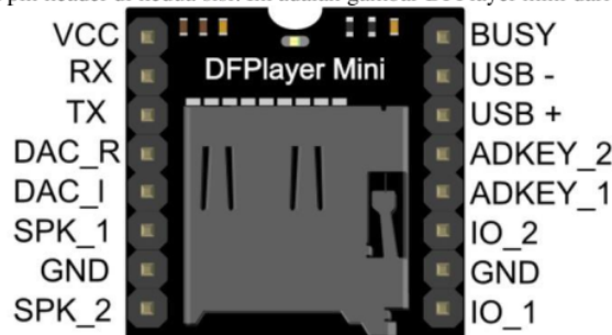
Gambar 3. Pin out DF Player
