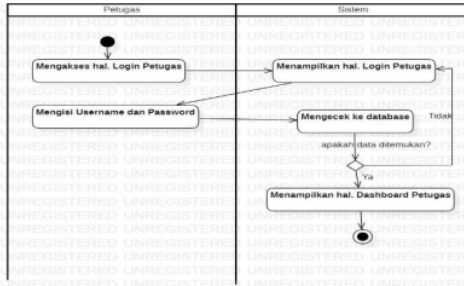
Gambar 14. Diagram Activity Login Petugas
