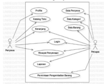
Gambar 5. Use Case Diagram SI InOutdoor rental
