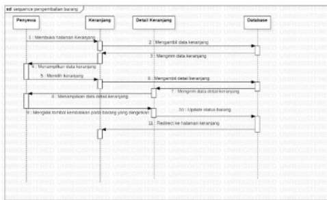
Gambar 10. Sequence Diagram Pengembalian Barang
