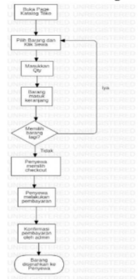
Gambar 3. Flowchart Sewa Barang
