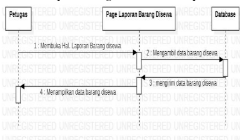
Gambar 9. Sequence Diagram Generate Laporan
