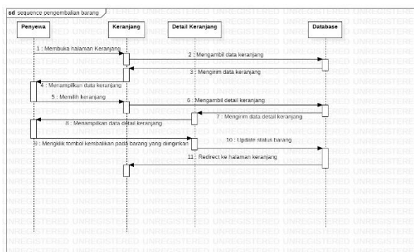
Gambar 10. Sequence Diagram Pengembalian Barang
