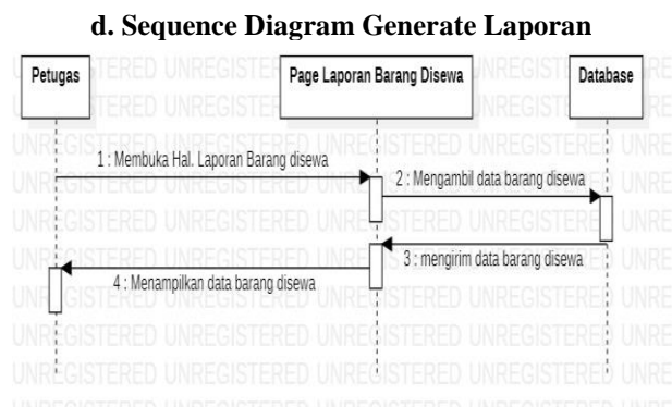
Gambar 9. Sequence Diagram Generate Laporan
