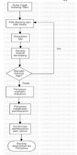
Gambar 3. Flowchart Sewa Barang
