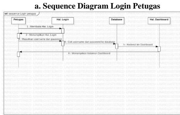
Gambar 6. Sequence Diagram Login Petugas
