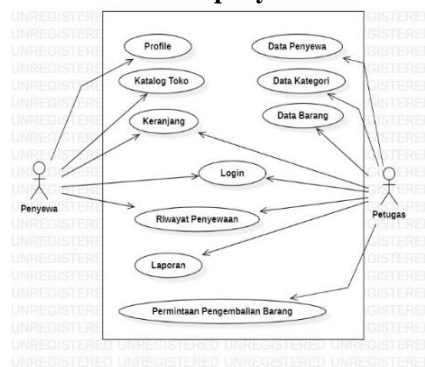
Gambar 5. Use Case Diagram SI InOutdoor rental
