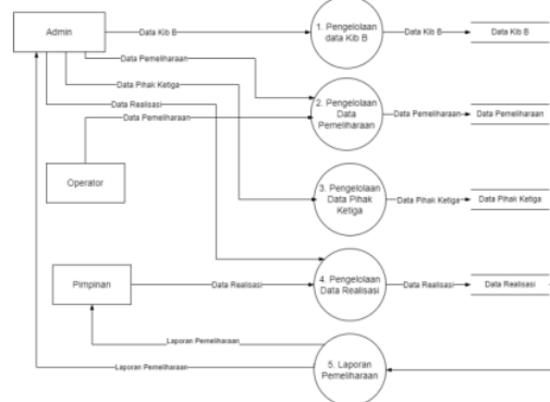
Gambar 5. DFD Level 1
