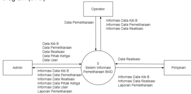
Gambar 4. DFD Level 0
