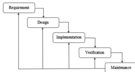
Gambar 1. Bagan Waterfall [15]
