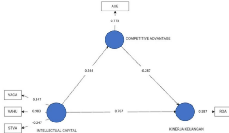
Gambar 2. 1 Hasil Bootstraping
