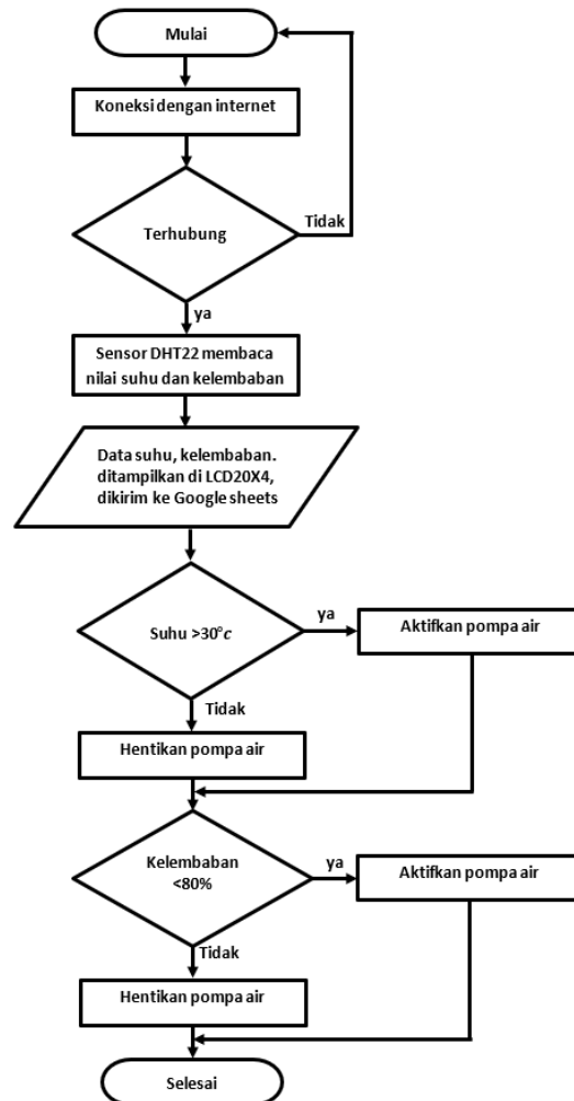
Gambar 2. Flowchart Sistem
