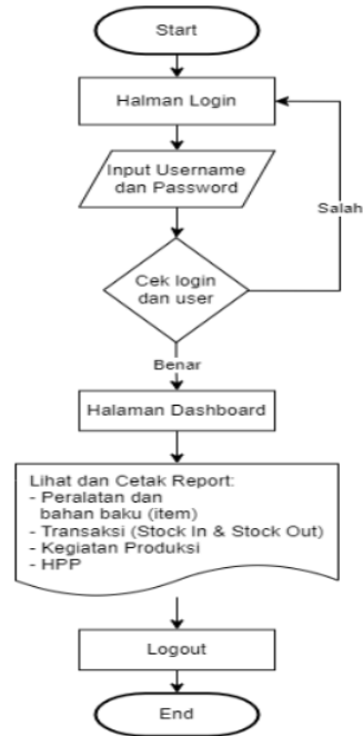
Gambar 3. Flowchart Owner
