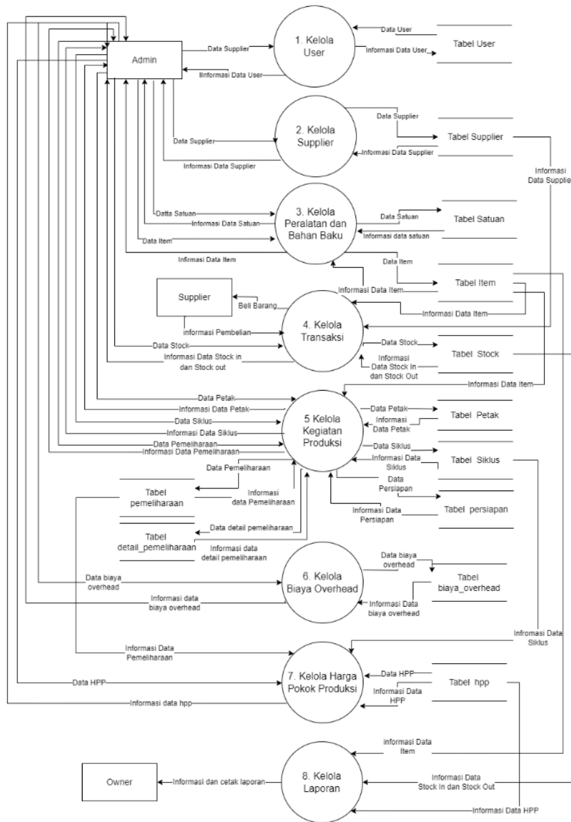
Gambar 5. DFD Level 1
