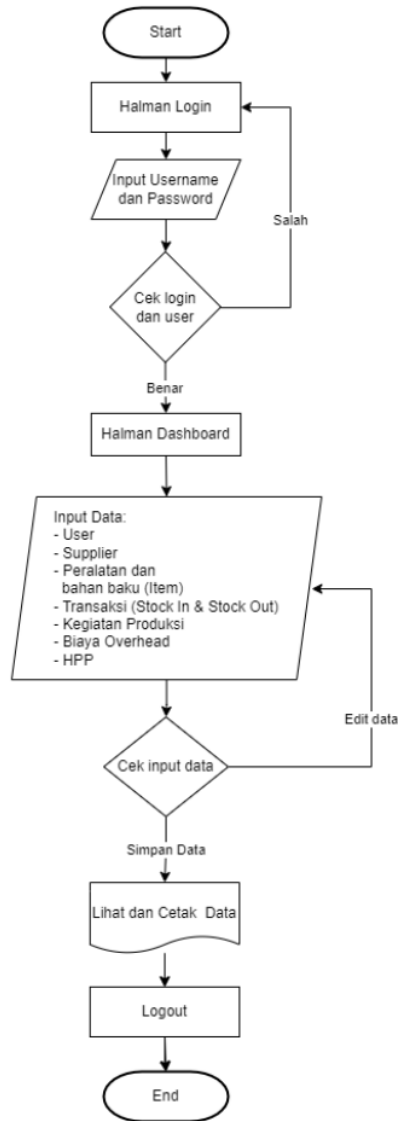
Gambar 2. Flowchart Admin
