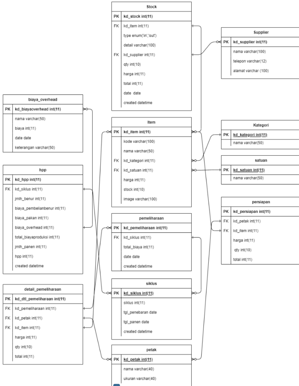
8 Gambar 6. Entity Relationship Diagram (ERD)
