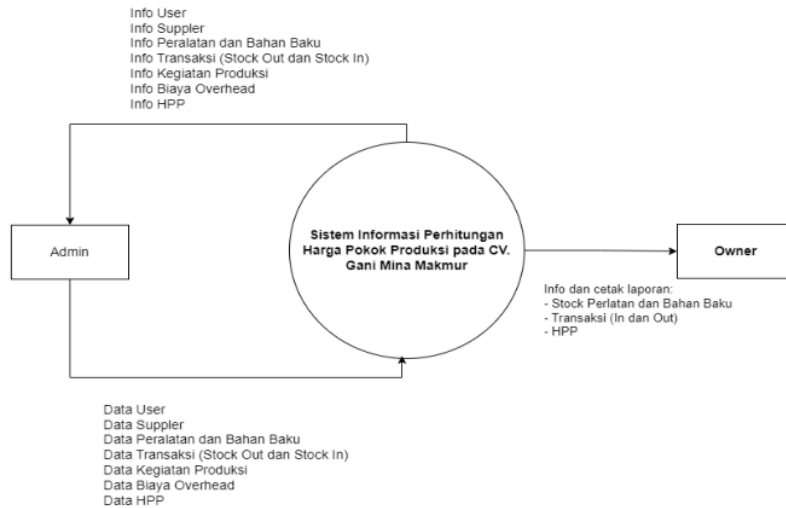
Gambar 4. DFD Level 0
