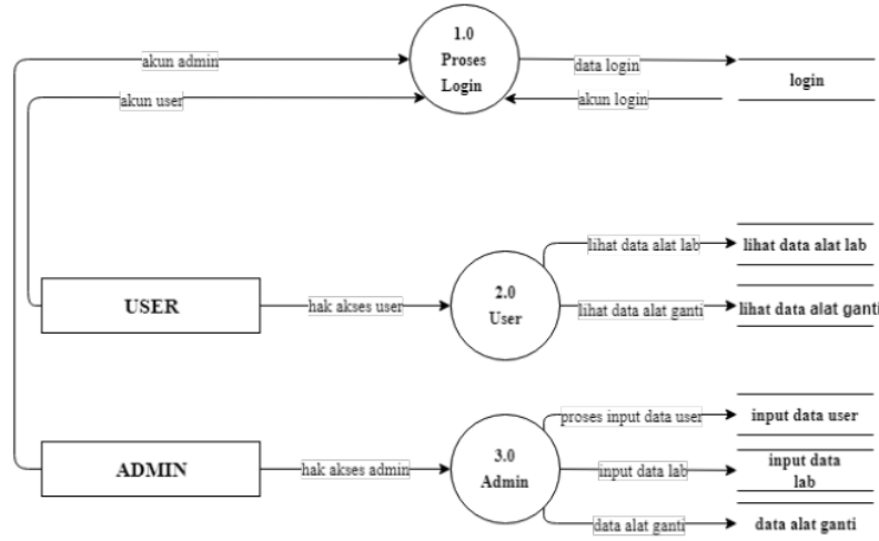
Gambar 6. Data Flow Diagram level 1
