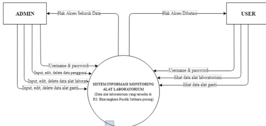
Gambar 5. Data Flow Diagram level 0
