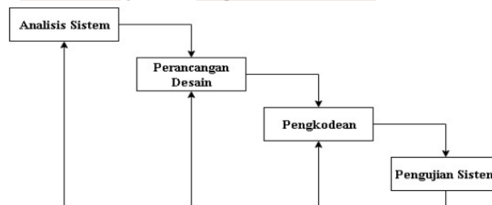
Gambar 1. Metode Waterfall
