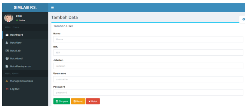
Gambar 9. Input User
