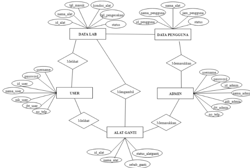
Gambar 4. Entity Realationship Diagram
