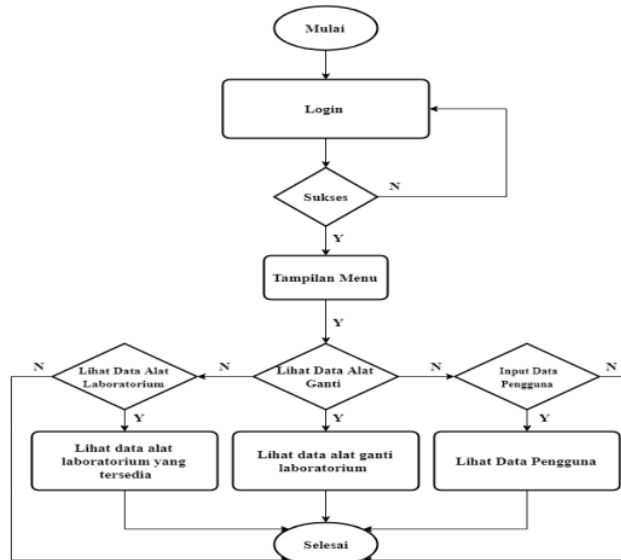
Gambar 3. Flowchart User
