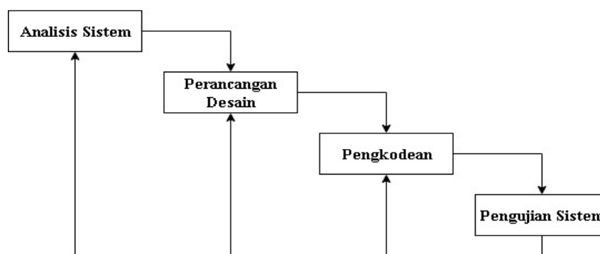
Gambar 1. Metode Waterfall
