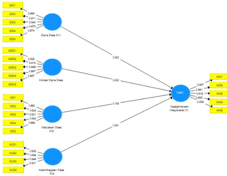
Gambar 2. Inner Output SmartPLS
