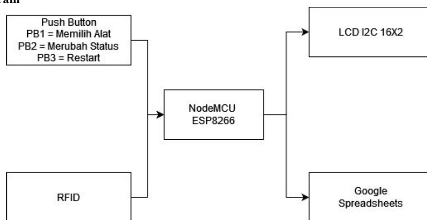
Gambar 2. Blok Diagram
