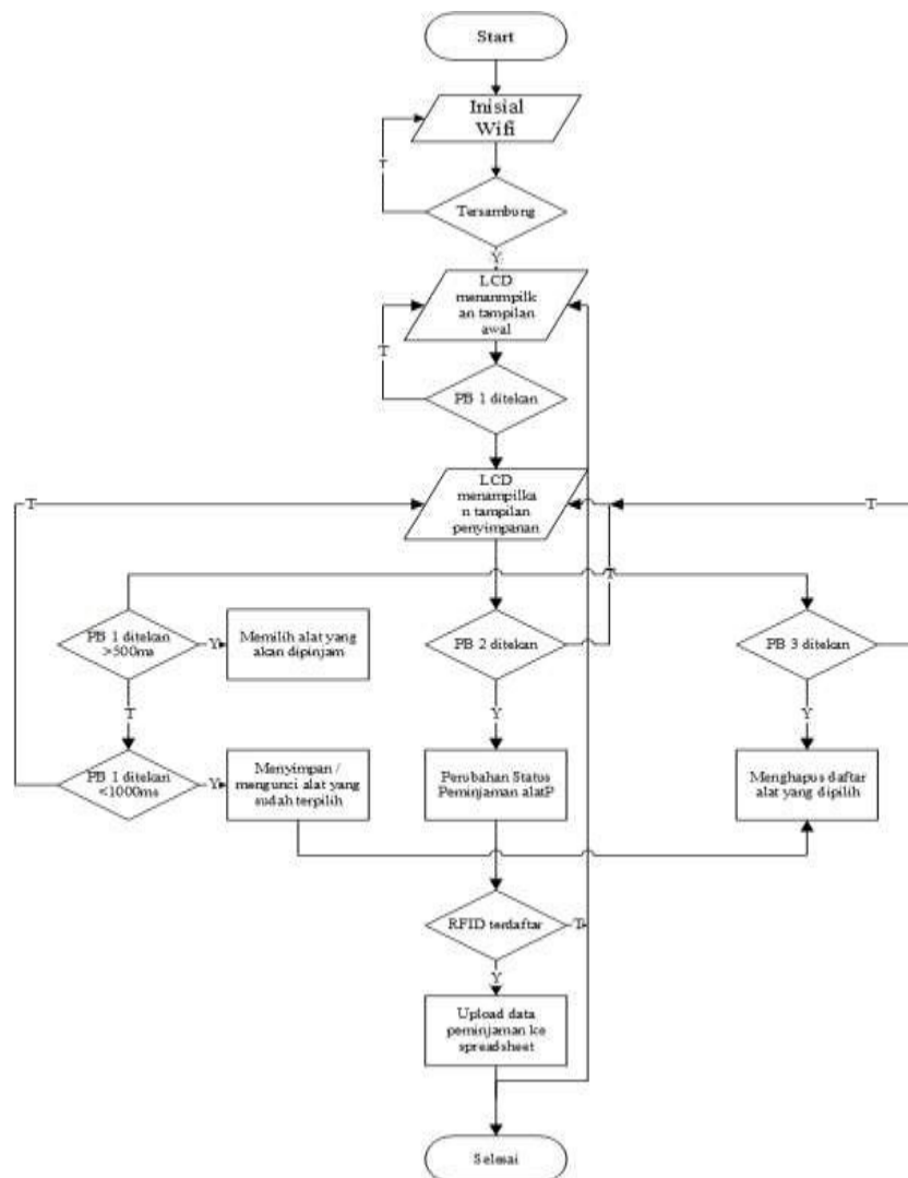
Gambar 1. Flowchart Sistem
