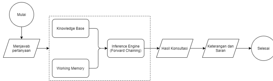
Gambar 1. Langkah-Langkah Metode Forward Chaining
