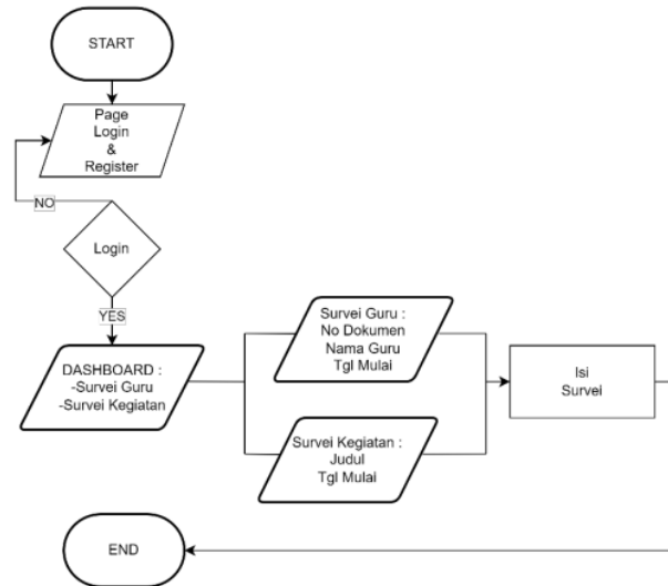
Gambar 3. Flowchart User
