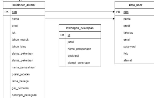
Gambar 5 Entity Relation Diagram(ERD)
