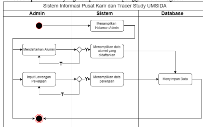
Gambar 3 Activity Diagram Admin
