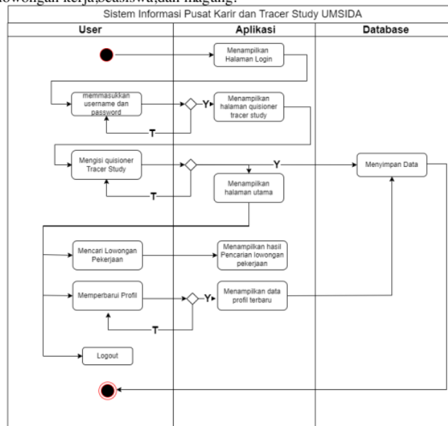
Gambar 4 Activity Digram User
