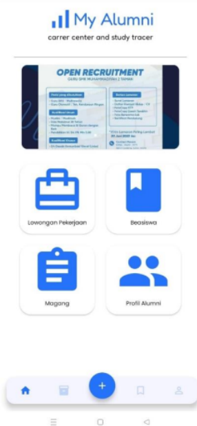
Gambar 10 Halaman Dashboard
