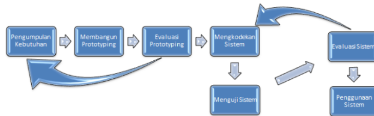
Gambar 1 Metode Prototype
