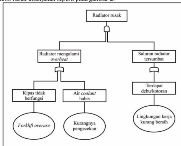
Gambar 2. FTA Radiator Rusak
