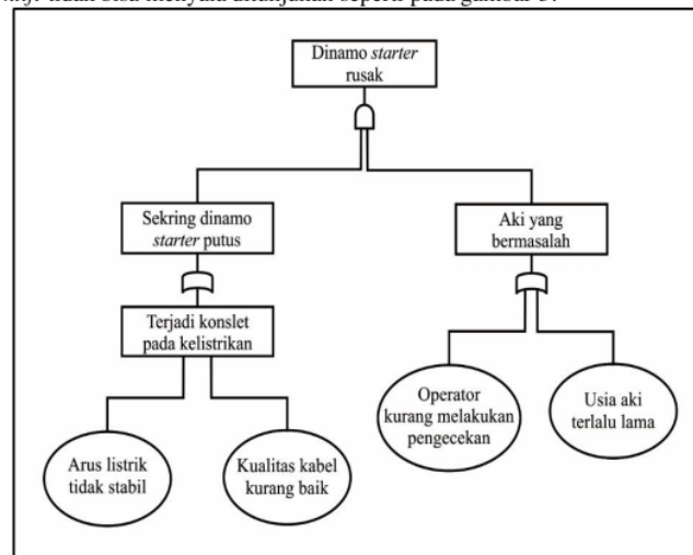
Gambar 3. FTA Dinamo Starter Rusak
