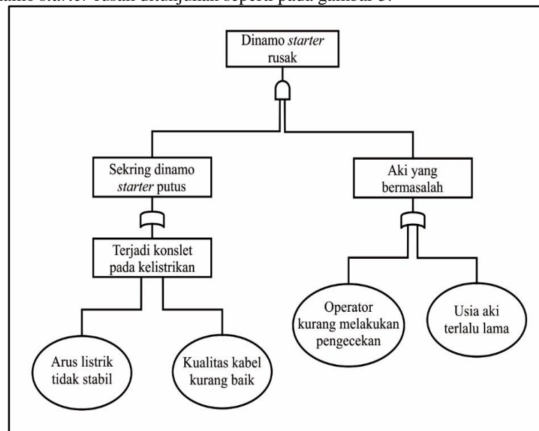
Gambar 3. FTA Dinamo Starter Rusak
