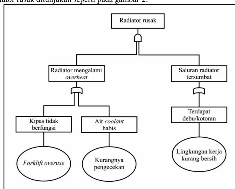
Gambar 2. FTA Radiator Rusak
