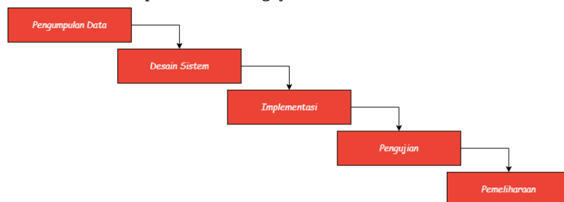
Gambar 1. Metode Waterfall
