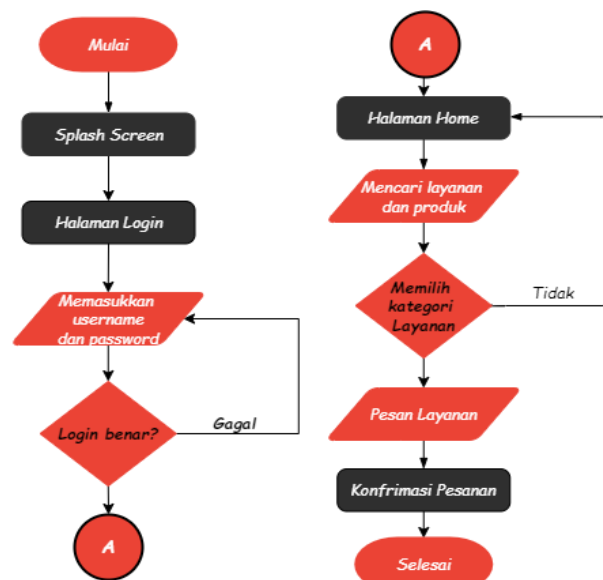
Gambar 2. Flowchart
