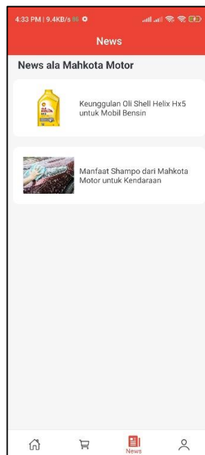
Gambar 14. Halaman News
