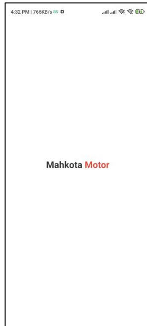
Gambar 5. Splash Screen
