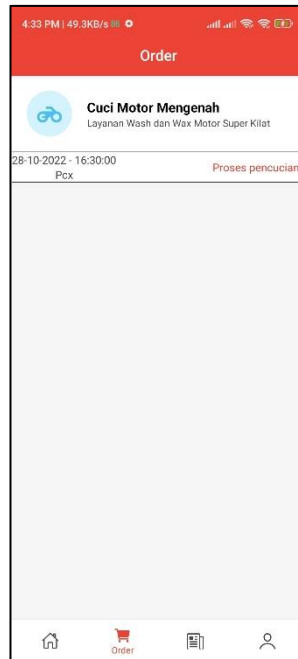
Gambar 13. Halaman Order
