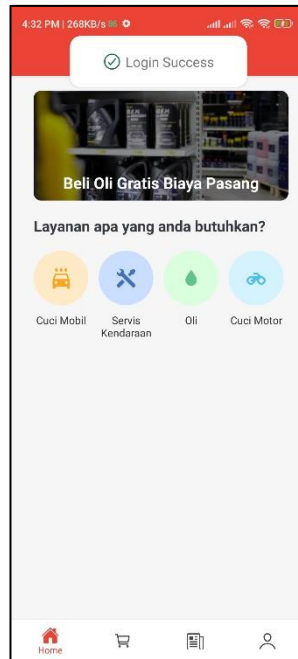
Gambar 7. Halaman Home
