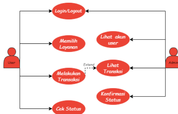
Gambar 3. Usecase Diagram
