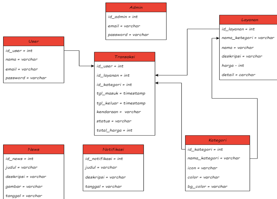
Gambar 4. Database Diagram
