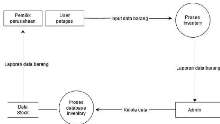
Gambar 3 DFD Level 1
