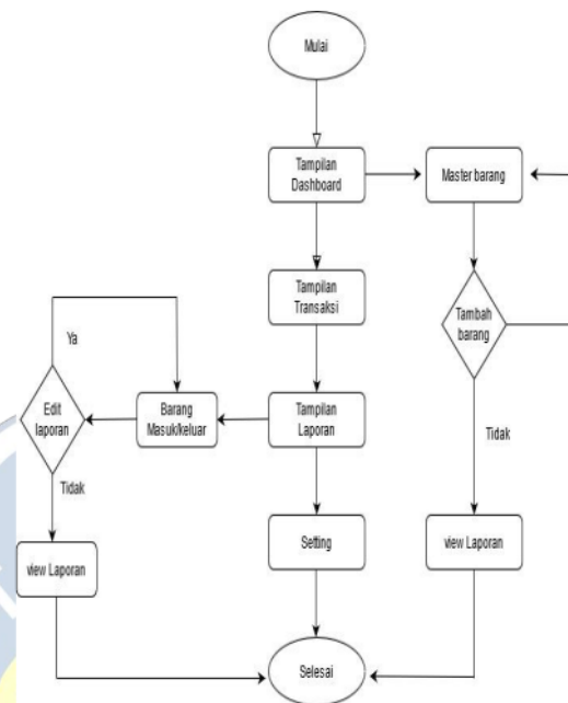
Gambar 1 Flowchart Sistem
