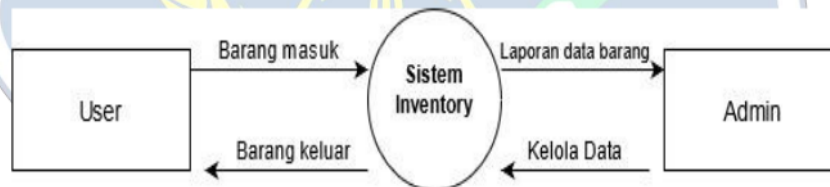
Gambar 2 DFD Level 0
