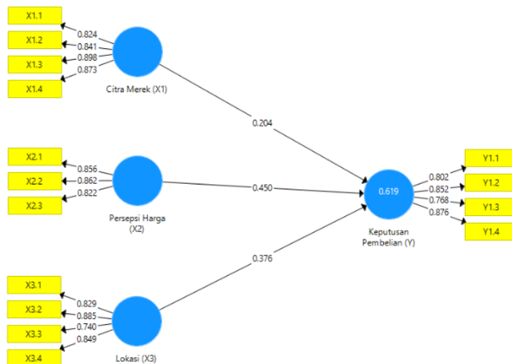
Gambar 2. Loading Factor Sumber: Pengolahan Data (SPLS, 2022)
