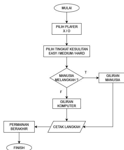
Gambar 3. Flowchart Permainan Game Tic-Tac-Toe
