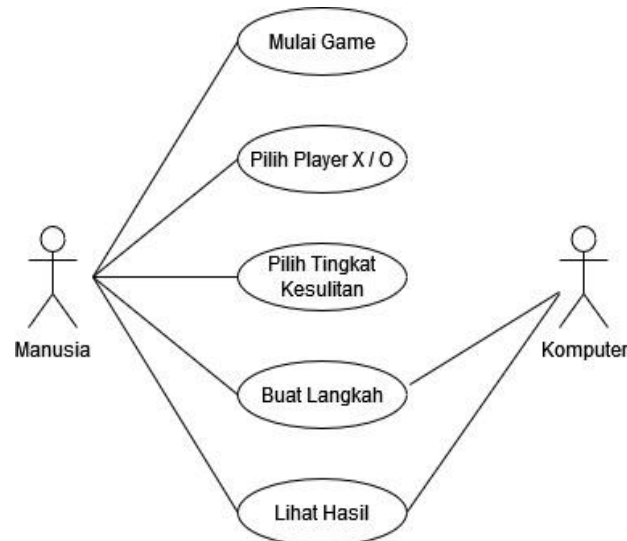
Gambar 4. Use Case Diagram Permainan Game Tic-Tac-Toe
