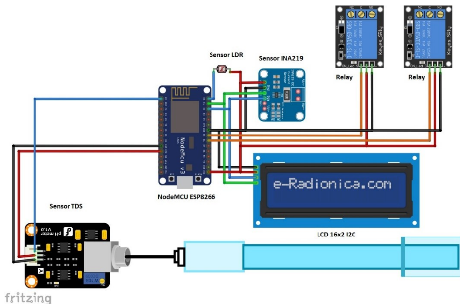
Gambar 3. Wiring Diagram
