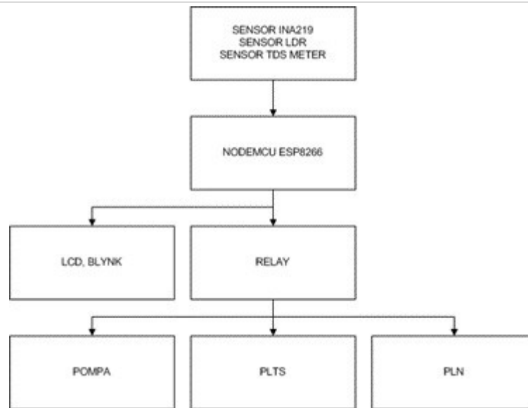
Gambar 2. Diagram Blok
