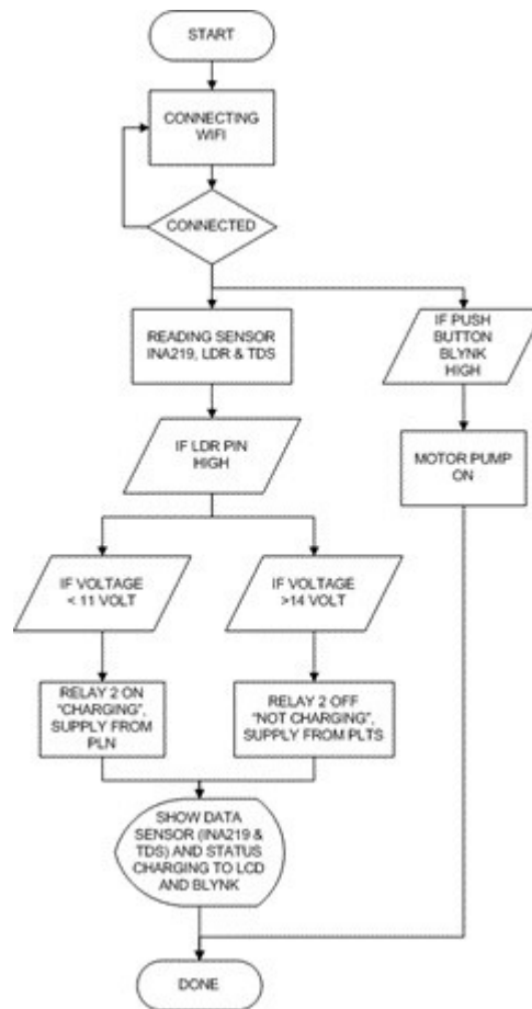
Gambar 1. Flowchart Sistem
