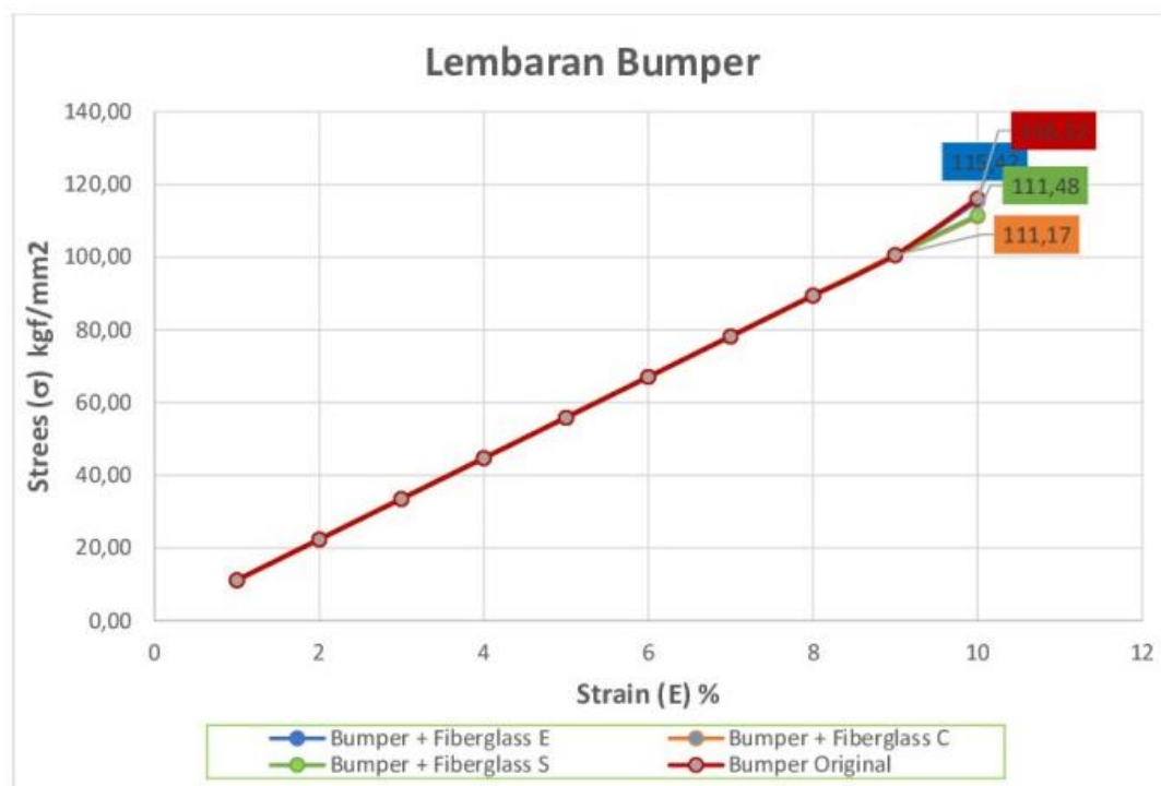
Gambar 2. Grafik Rata-Rata Uji Bending Bumper Mobil
