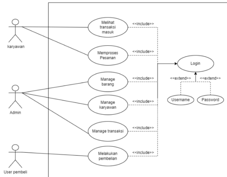
Gambar 5. Use Case Diagram
