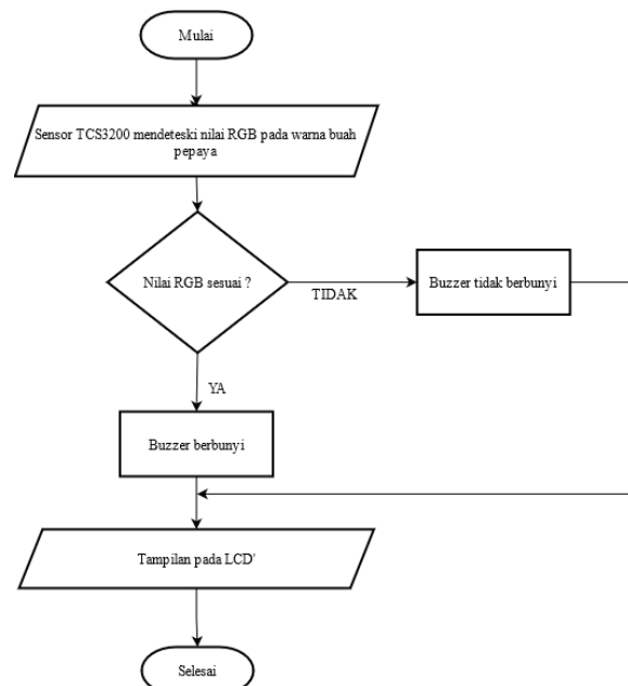
Gambar 3. Flowchart Program
