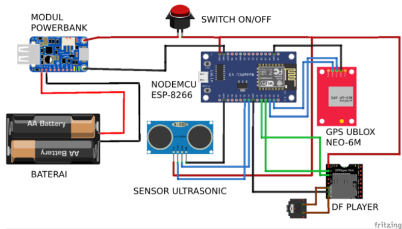
Gambar 3. Wiring Diagram
