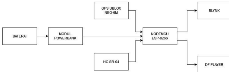
Gambar 2. Blok Diagram
