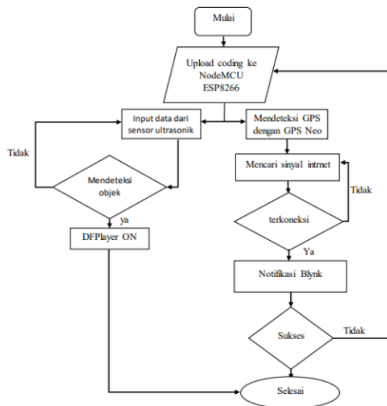
Gambar 1. Flowchart Sistem
