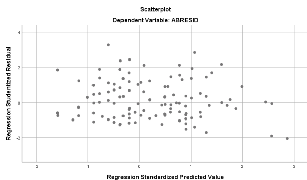
Gambar 1. Scatterplot
