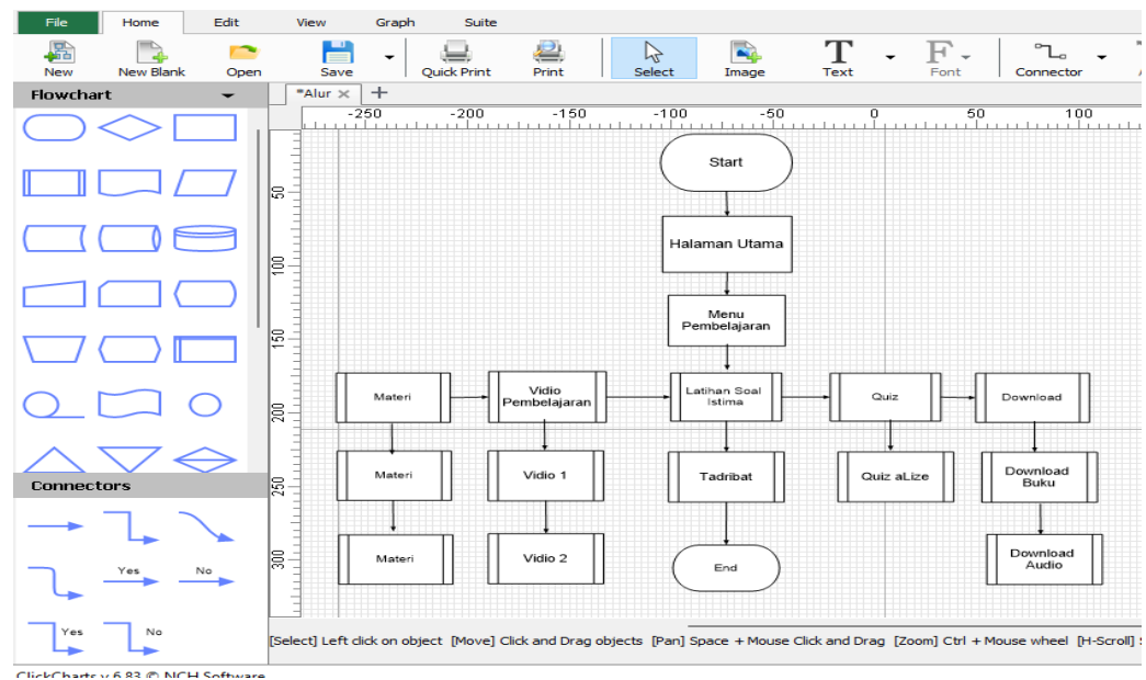
Gambar. flowchart
