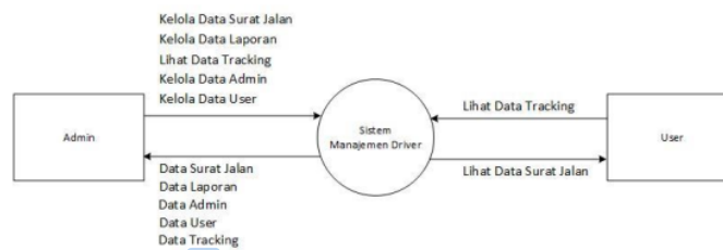
Gambar 3. Data Flow Diagram Level 0
