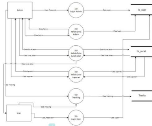
Gambar 4. Data Flow Diagram Level 1
