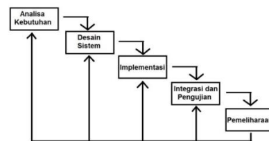
Gambar.1 Metode Waterfall
