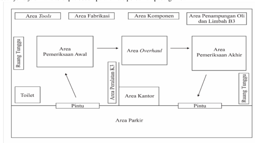
Gambar 2. Layout awal
