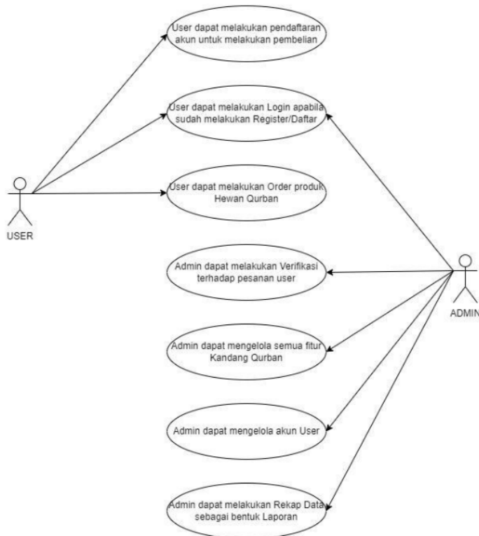
Gambar 5 Diagram Use Case
