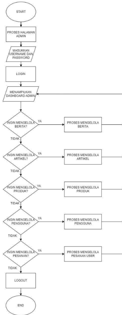
Gambar 3 Flowchart Admin
