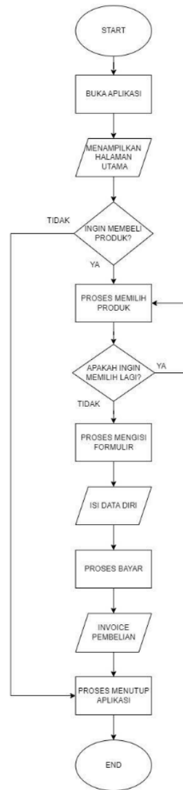
Gambar 2 Flowchart user
