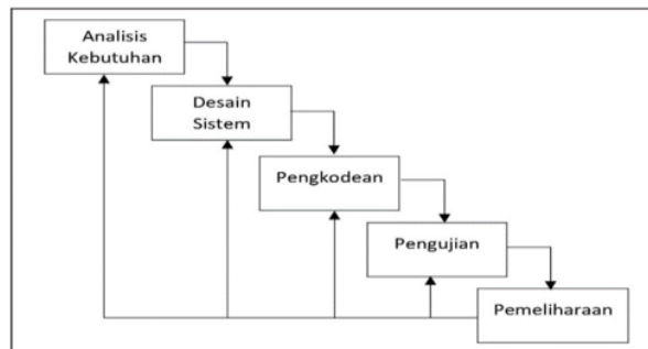
Gambar 1 Bagan Waterfall
