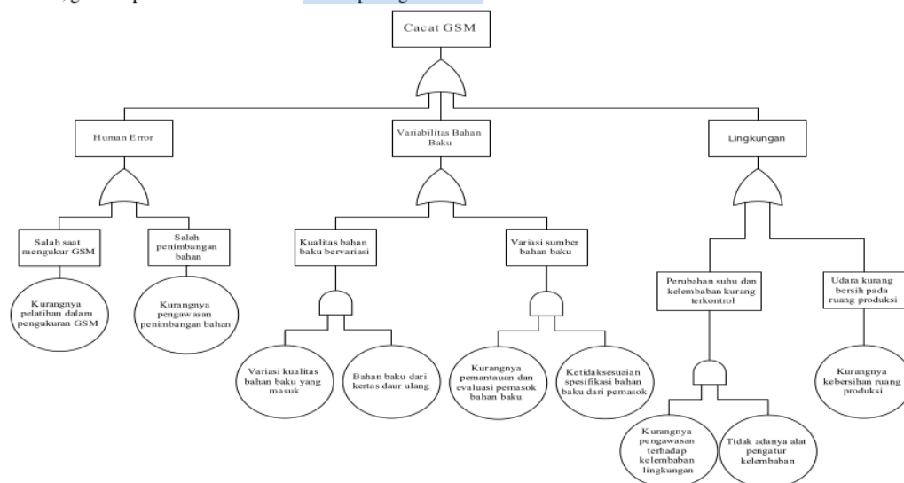
Gambar 2. Fault Tree Analysis cacat GSM
