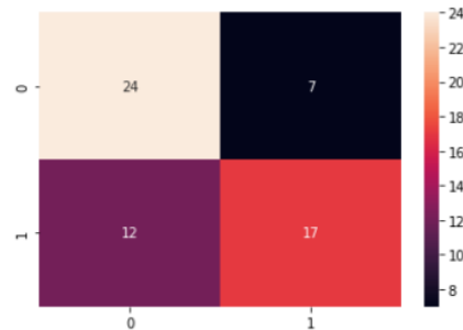
Gambar 4 Confusion Matrix
