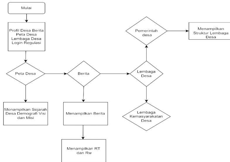
Gambar 2.Flowchat
