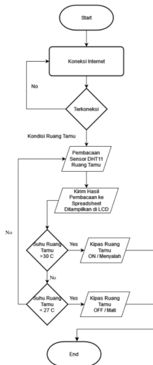
Gambar 4. Flowchart Ruang Tamu
