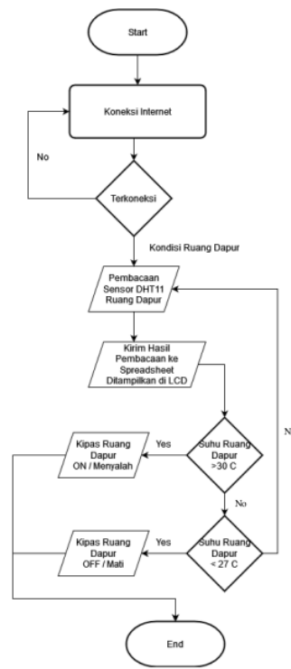
Gambar 5. Flowchart Ruang Dapur
