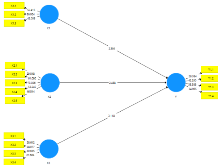
Gambar 1. Bootstrapping Test Results
