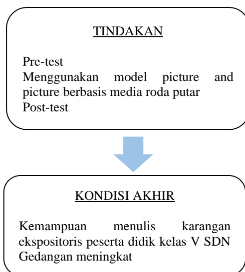
Gambar 2.1 alur penelitian
