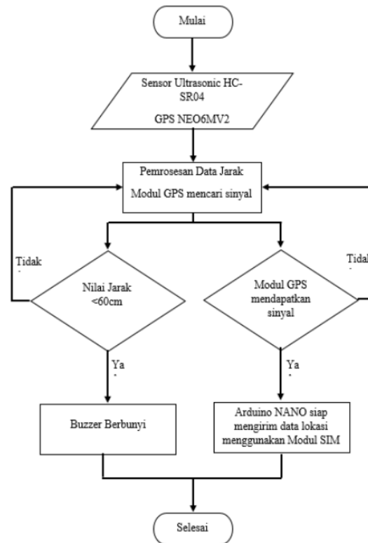
Gambar 13. Flow Chart Sistem
