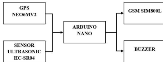
Gambar 12. Blok Diagram
