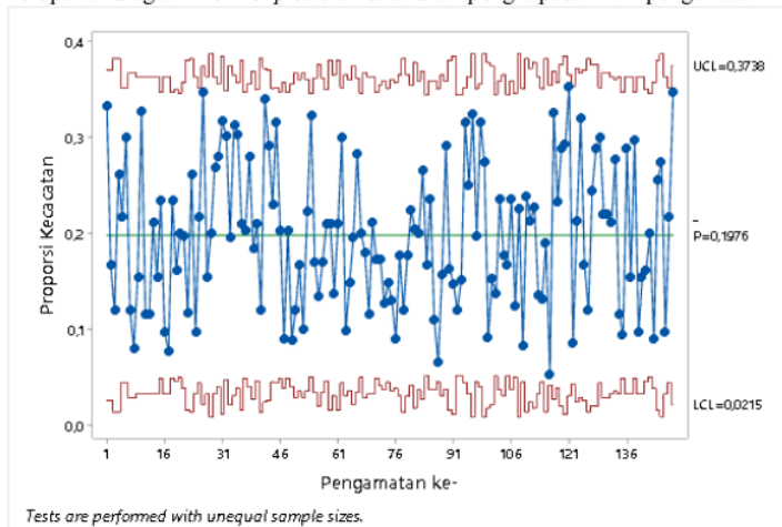
Gambar 7. Diagram Kontrol Proporsi ( p ) (Iterasi 1)
