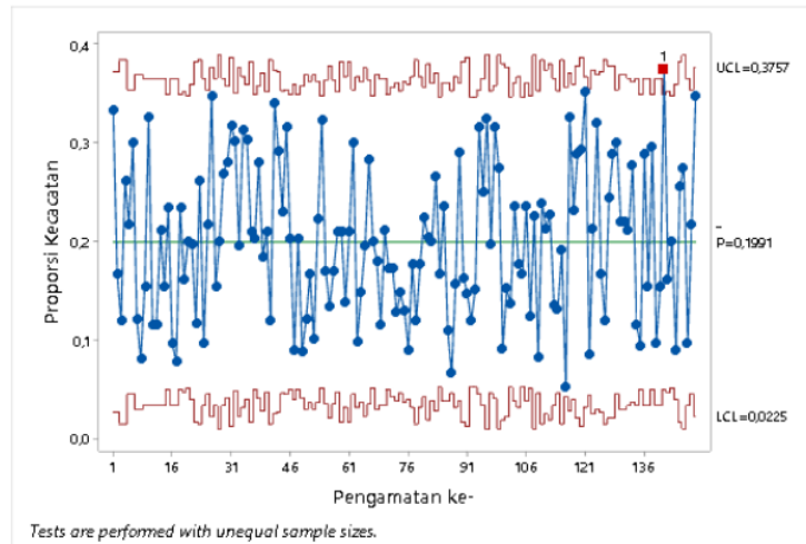
Gambar 6. Diagram Kontrol Proporsi ( p )
