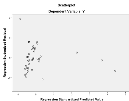
Gambar 3 : Scatterplot
