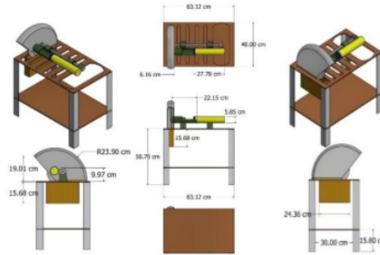
Gambar 3. Design Drawing .
