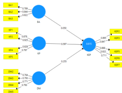
Gambar 4. Nilai factor loading model akhir
