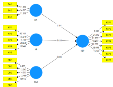
Gambar 3. Nilai factor loading model awal
